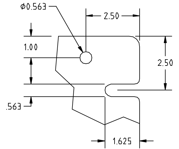
CORNER DETAIL
