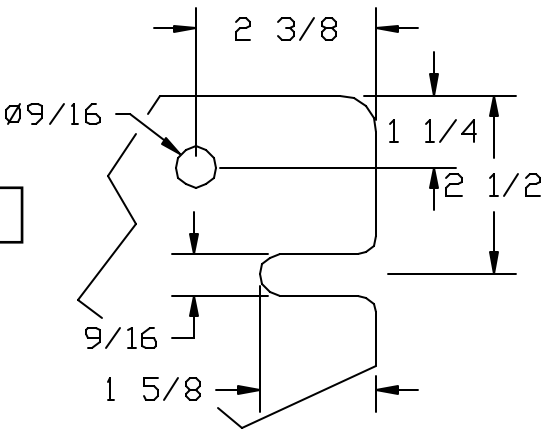
CORNER DETAIL
