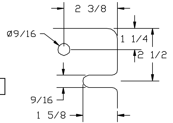
CORNER DETAIL
